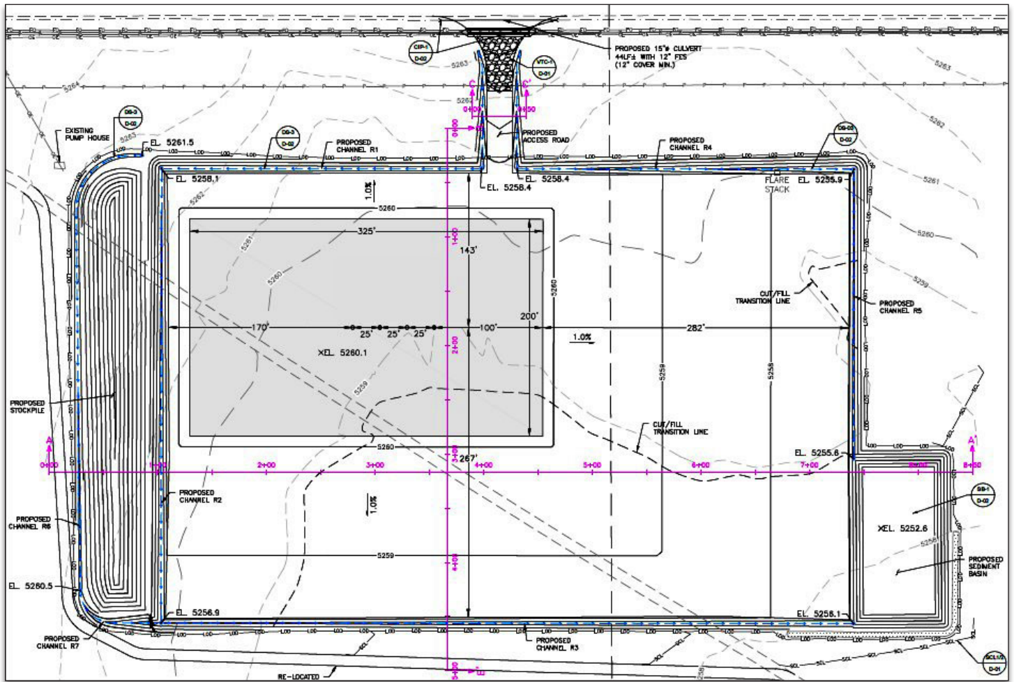
Site Grading Plan
